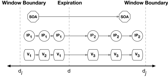
Fig. 5: Using different components to identify ownership changes.
