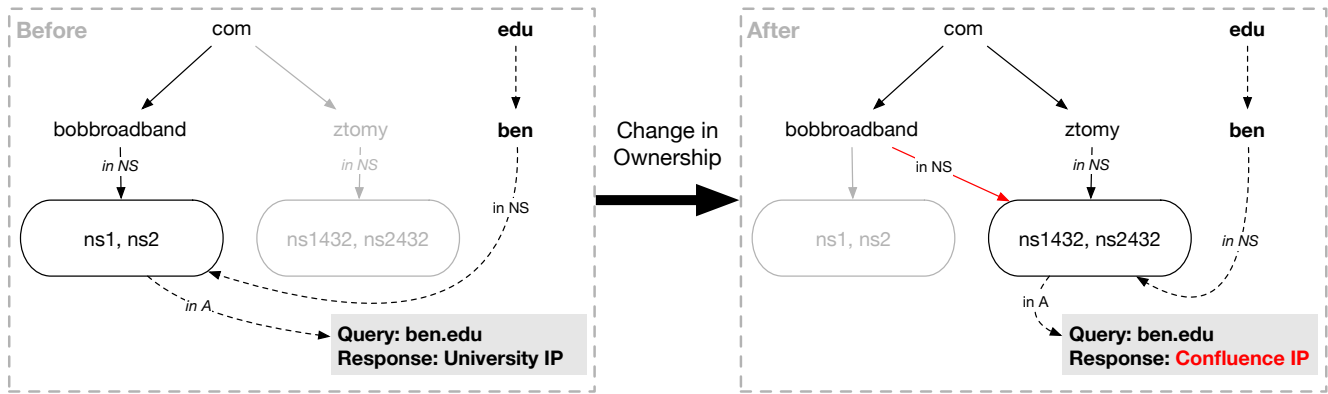
Fig. 2: Residual Trust Exploitation in University DNS Servers
